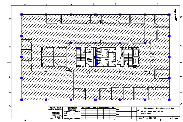
Office 3rd Story
